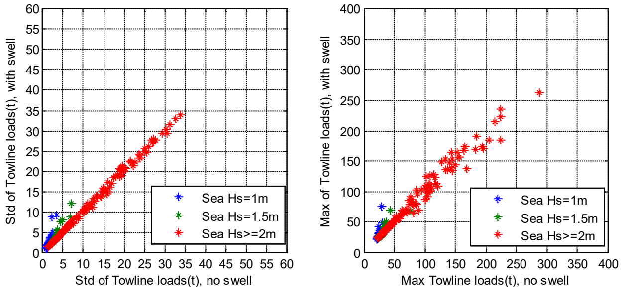
Figure 6-3: Comparison of std and max towline tensions with and without swell, 15 t tug
