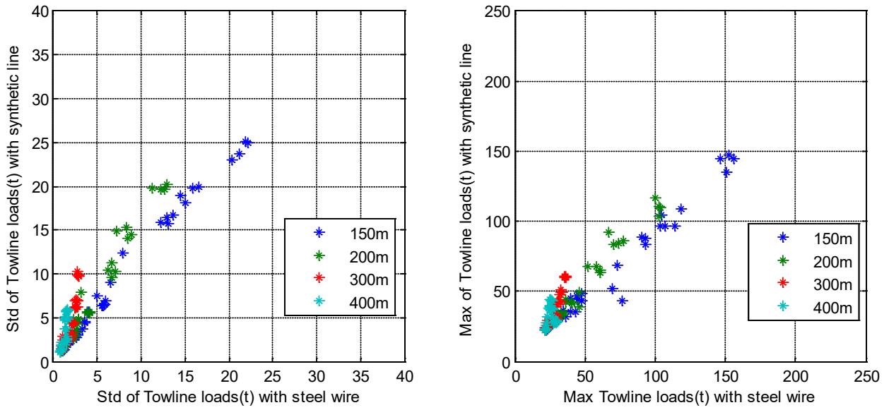
Figure 6-6: Comparison of std and max tensions for steel and synthetic towline, 15 t tug
