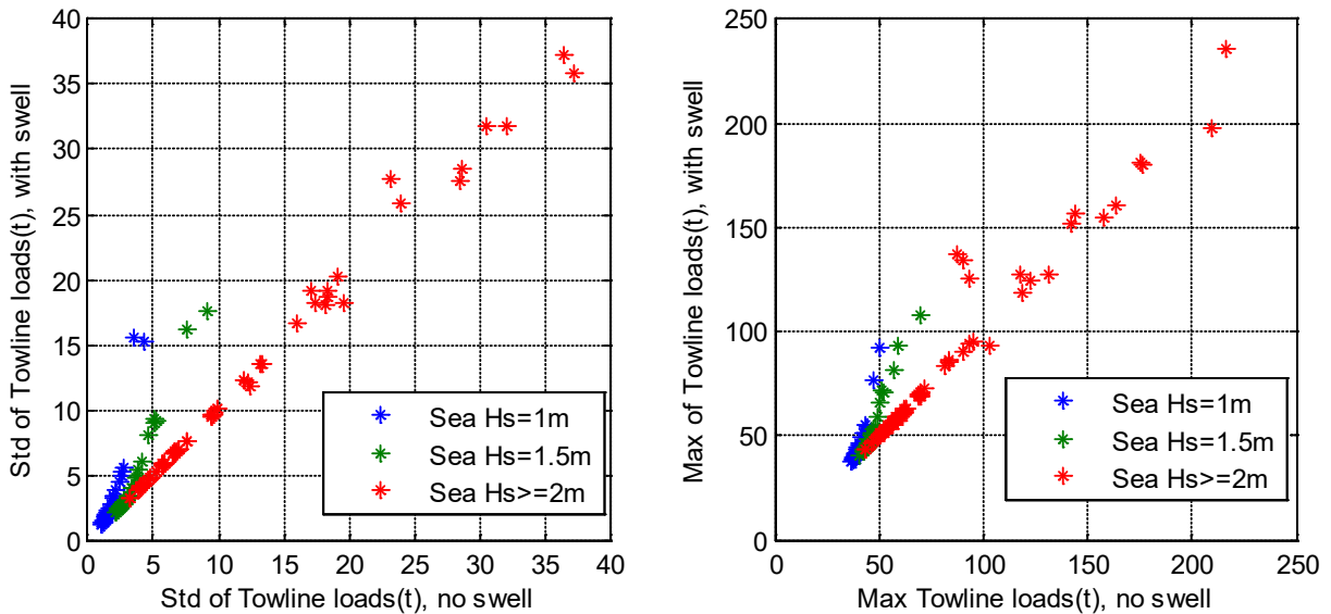
Figure 6-9: Comparison of std and max towline tensions with and without swells, 30 t tug
