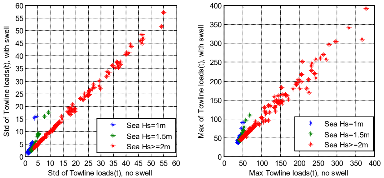
Figure 6-4: Comparison of std and max towline tensions with and without swell, 30 t tug
