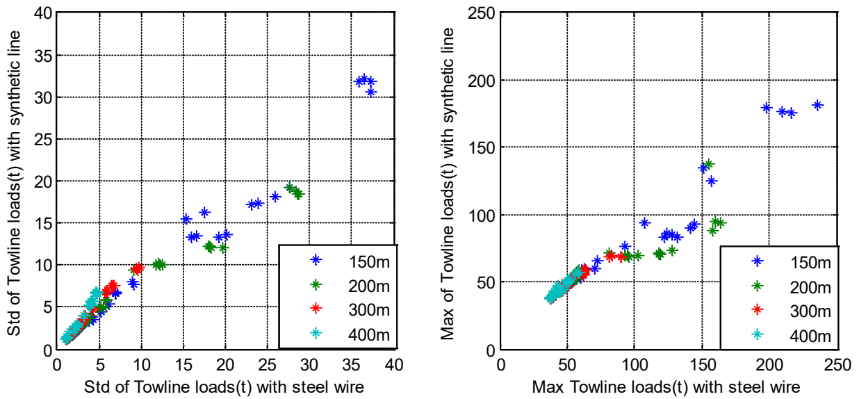
Figure 6-7: Comparison of std and max tensions for steel and synthetic towline, 30 t tug
