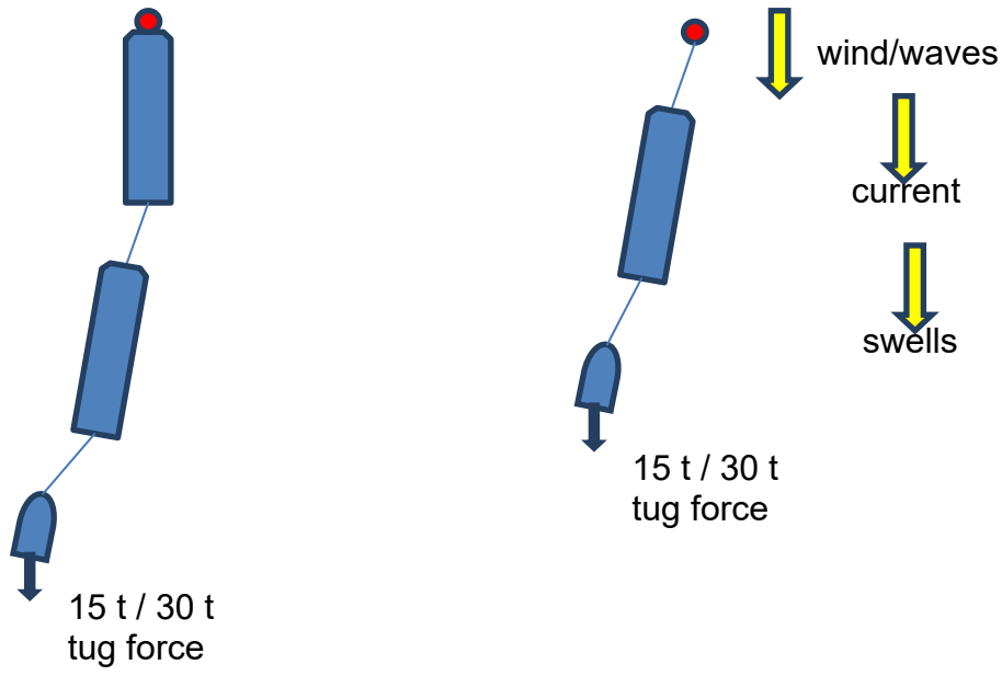
Figure 5-1: Schematic of the static tow operation with the FPSO and CALM buoy
