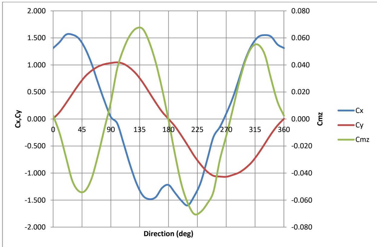
FIGURE 3 FPSO wind coefficients
