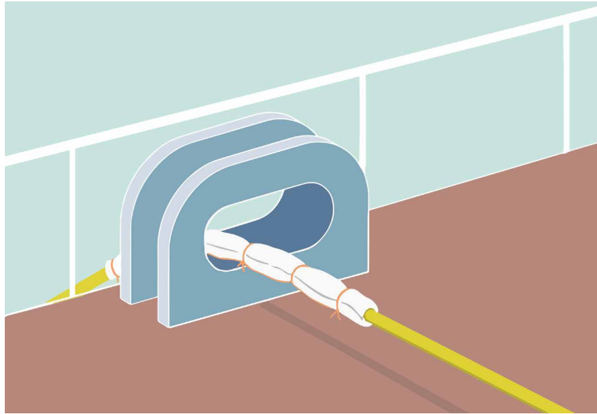
Figure 2.4: Chafe protection for HMSF towline pennant
