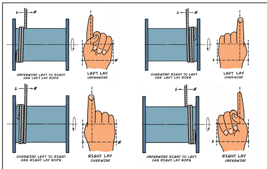
Figure 3.2: Correct installation of wire rope to winch drum
