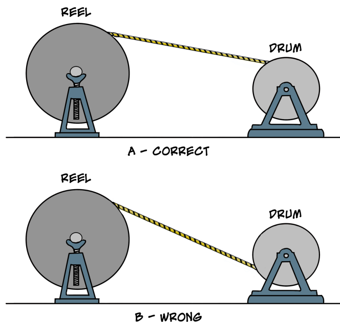
Figure 3.3: Installing a wire rope to a winch from a cable drum
