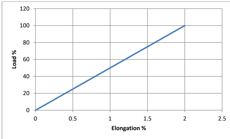
Figure 4-2: LEC curve of synthetic towline
