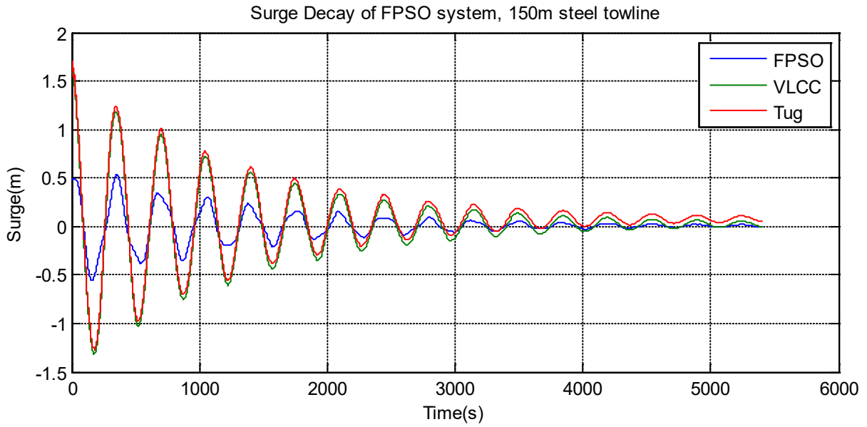
FIGURE 9 FPSO system, surge decay in calmwater
