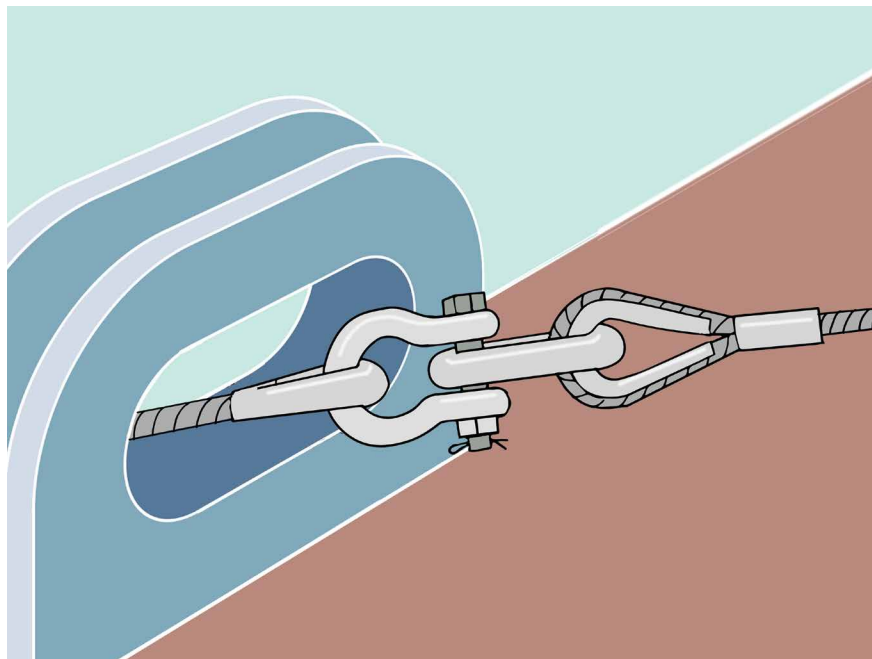
Figure 2.10: Towline assembly master link
