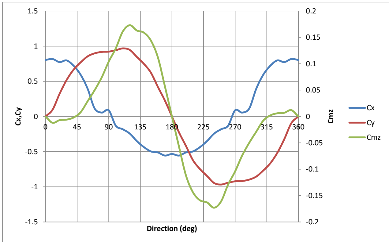
FIGURE 5 Tug wind coefficients
