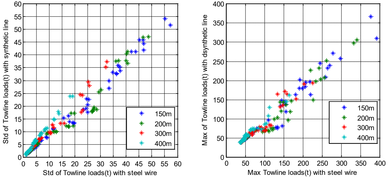
Figure 6-2: Comparison of std and max tensions for steel and synthetic towline, 30 t tug
