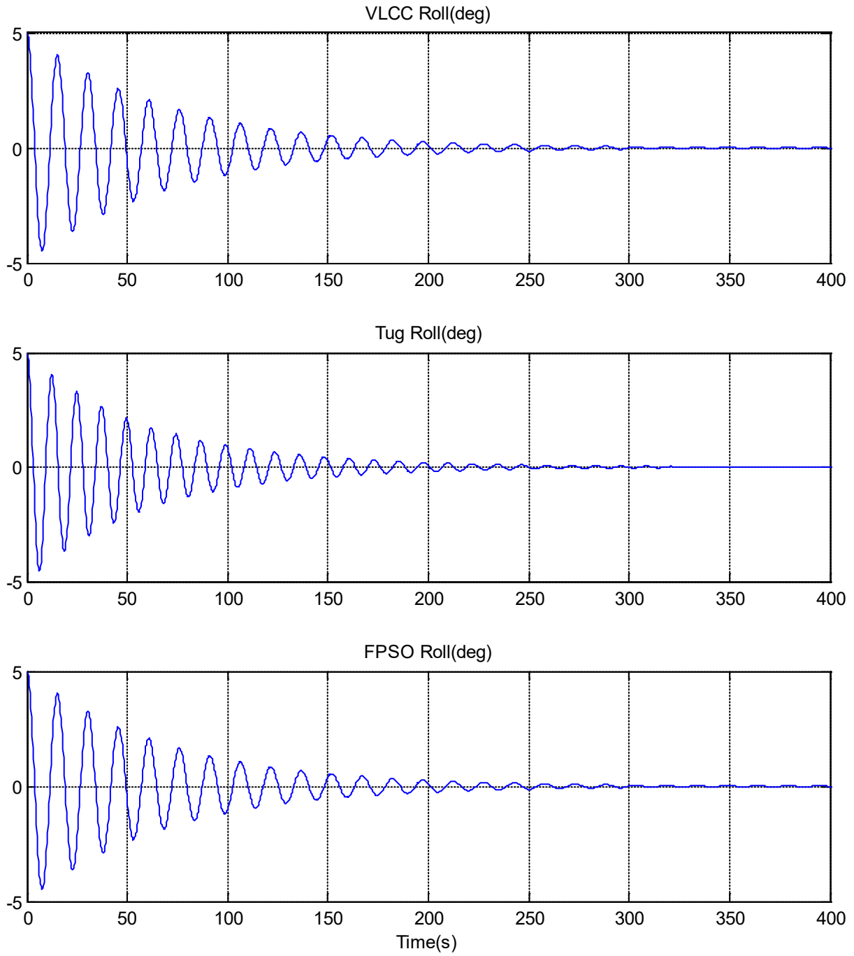
FIGURE 6 Roll decays
