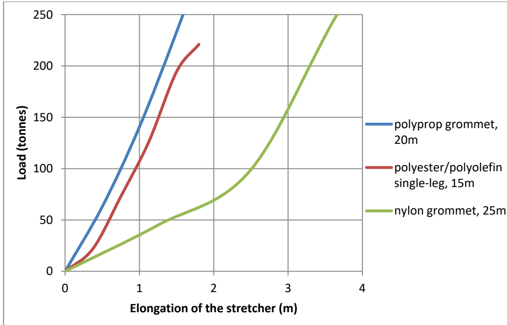
Figure 4-3: LEC curves for the 3 different stretchers
