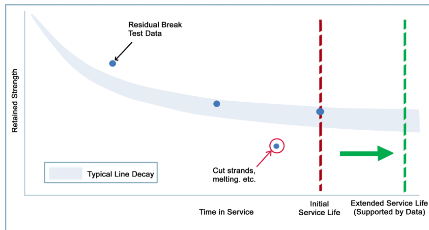
Figure 6.2: Example of a towline service life model
