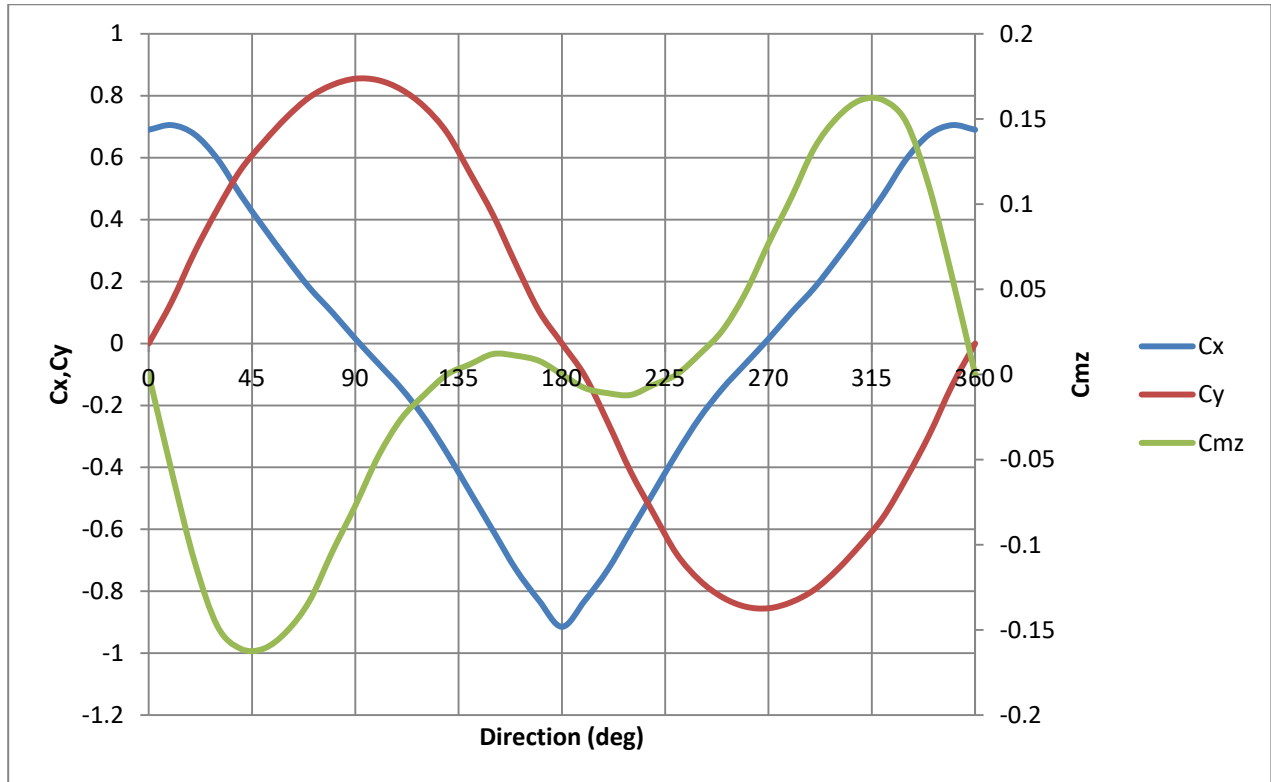
FIGURE 4 VLCC wind coefficients
