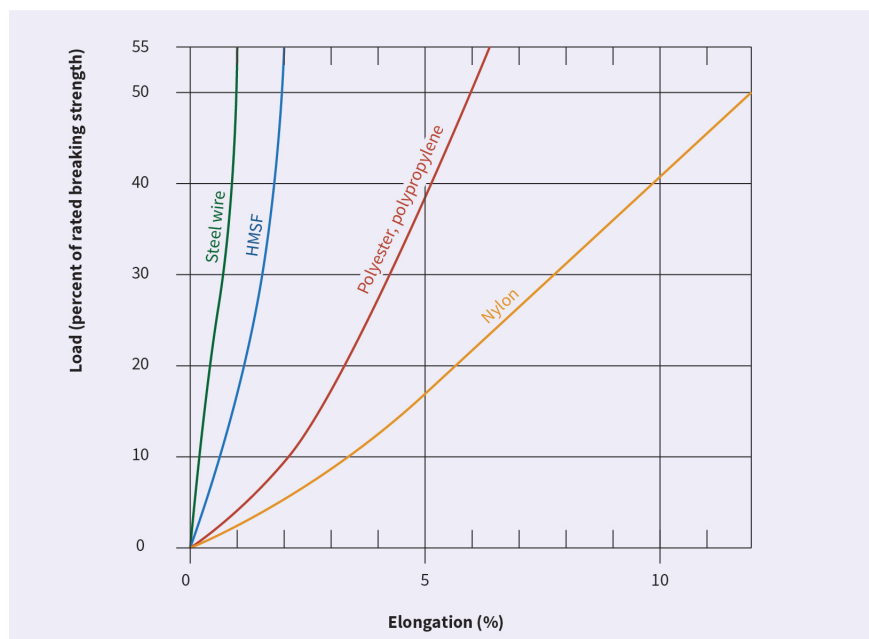
Figure 2.2: Typical load/extension stiffness characteristics of wire and synthetic fibre lines
