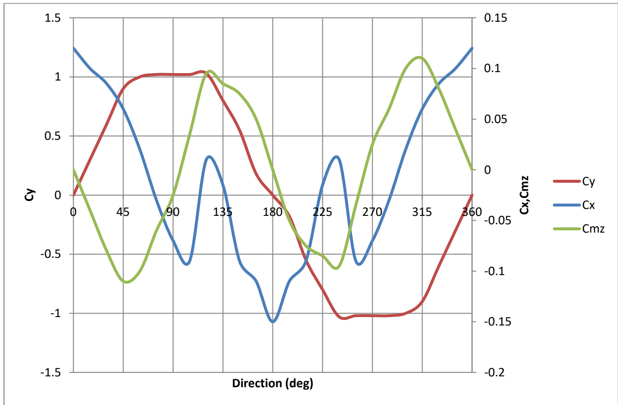
FIGURE 2 Tug current coefficients
