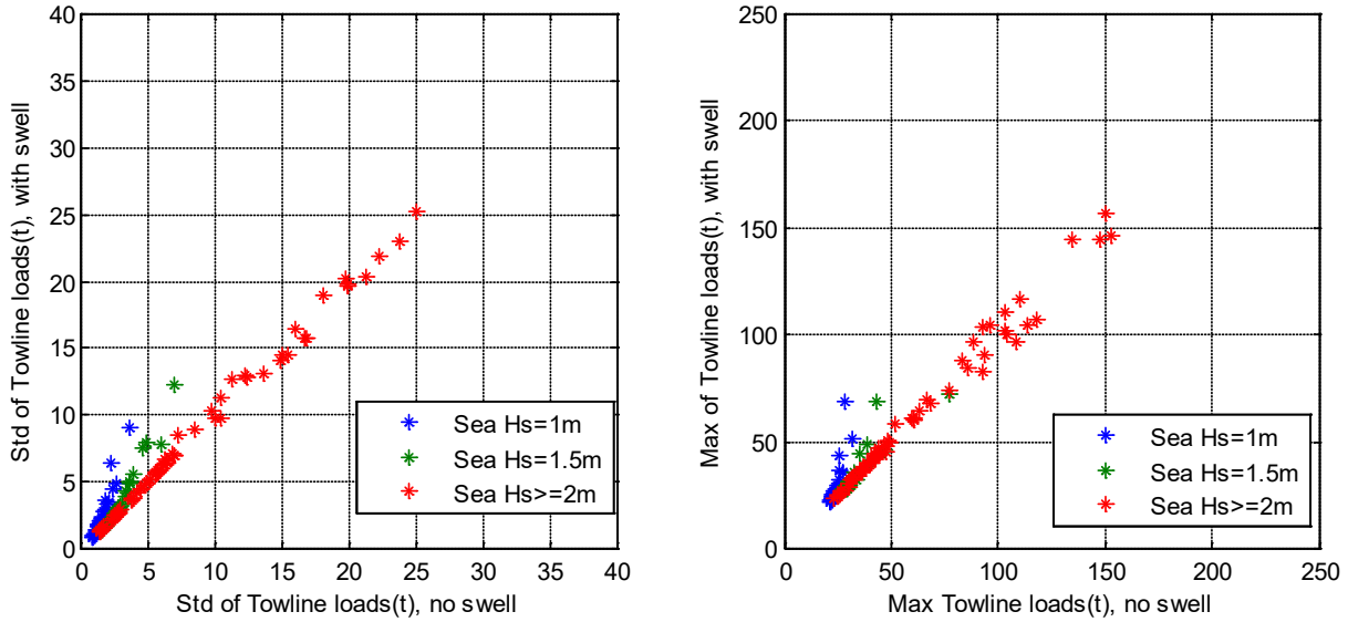
Figure 6-8: Comparison of std and max towline tensions with and without swells, 15 t tug
