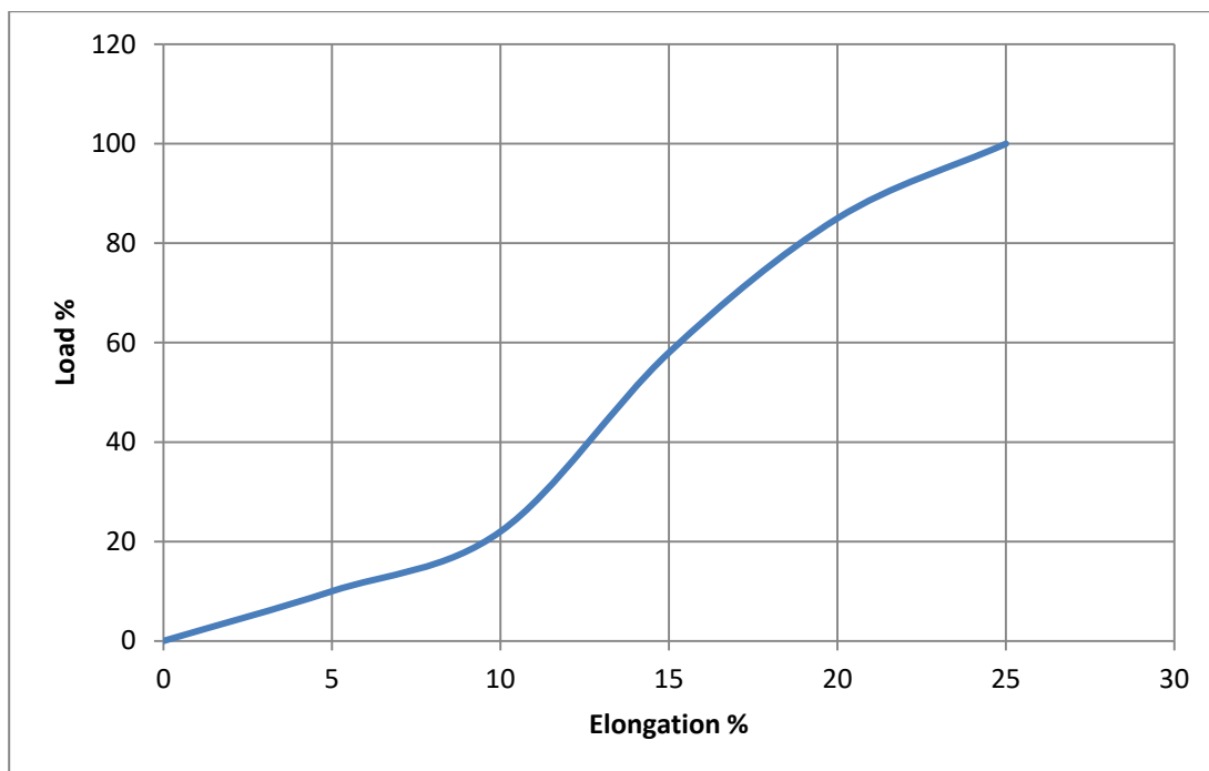
Figure 4-1: LEC curve of Nylon hawser
