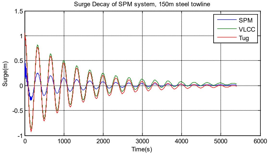
FIGURE 7 SPM system, surge decay in calmwater
