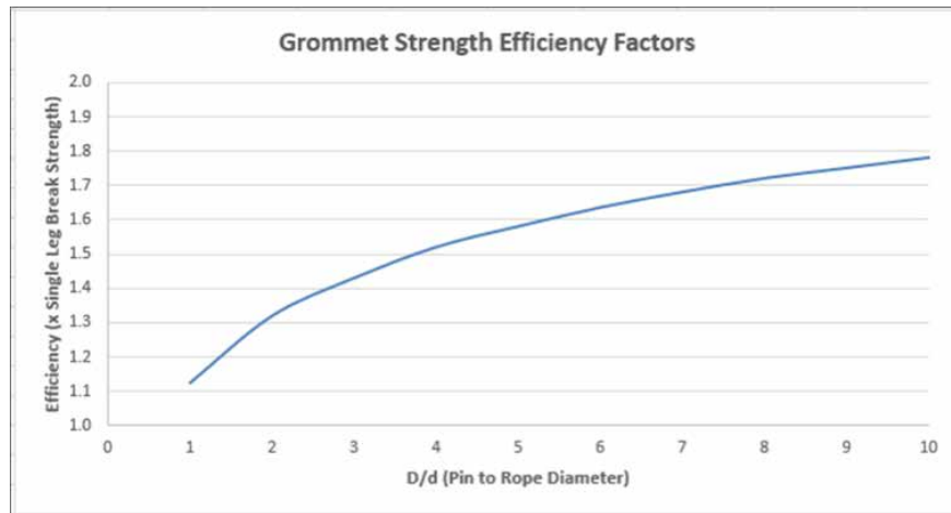
Figure 2.6: D/d efficiency factors
