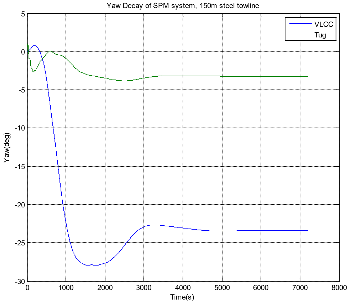
FIGURE 8 SPM system, yaw decay in current
