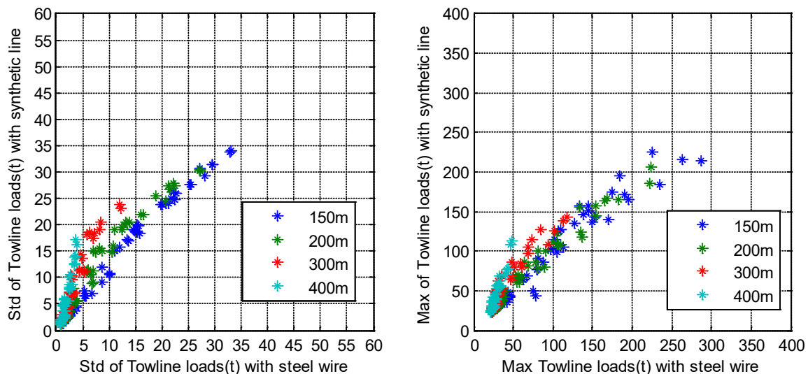
Figure 6-1: Comparison of std and max tensions for steel and synthetic towline, 15 t tug
