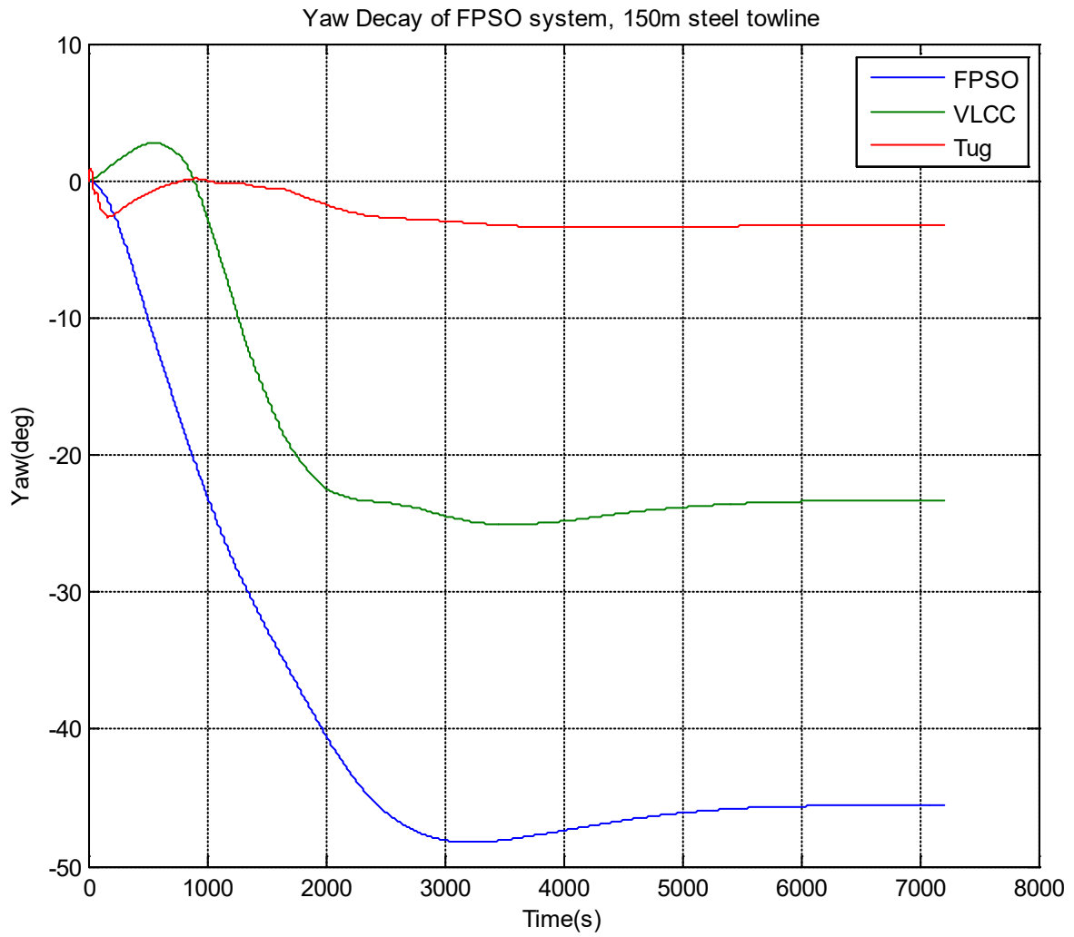
FIGURE 10 FPSO system, yaw decay in current
