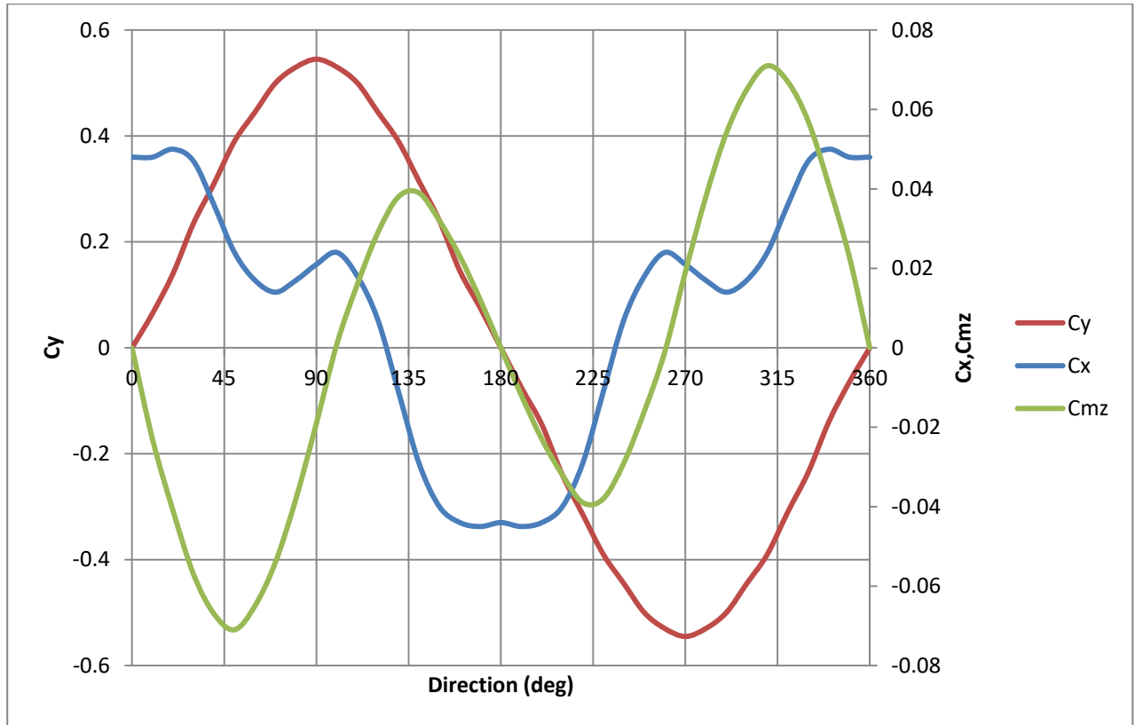
FIGURE 1 FPSO and VLCC current coefficients
