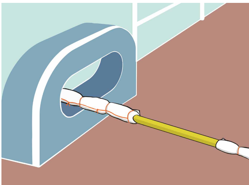
Figure 3.4: Synthetic towline pennant with chafing protection
