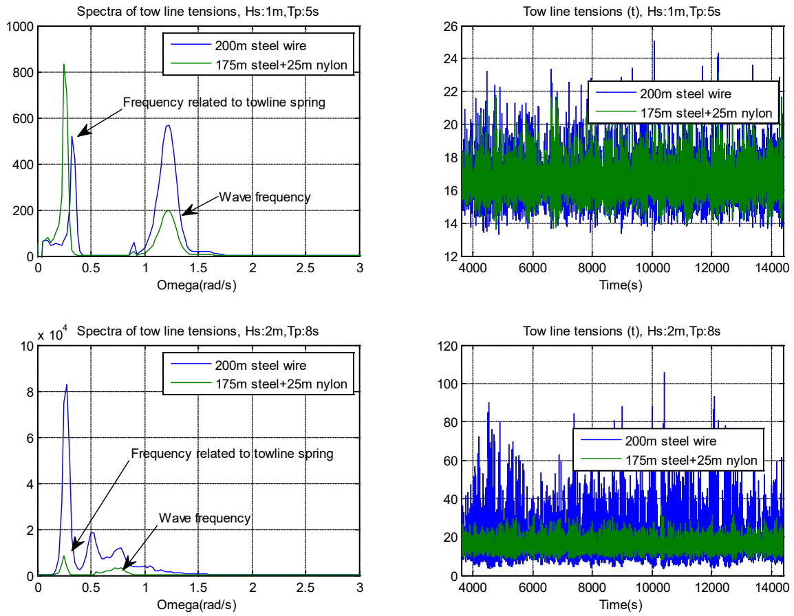
Figure 6-5: Comparison of tow line tensions with and without stretchers, 15 t tug
